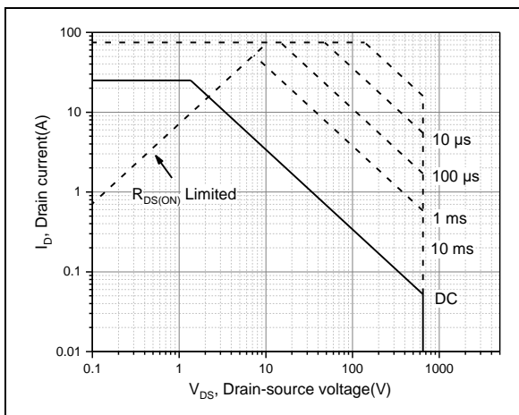
Figure 11, Safe operation area for TO220F T_C=25\text{ °C}
