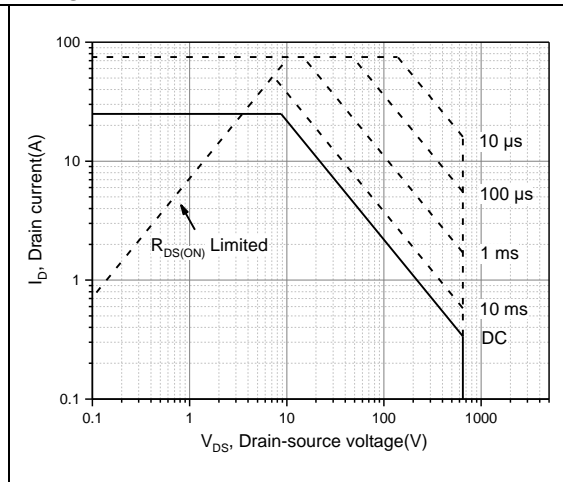
Figure 10, Safe operation area for TO263/TO247 T_C=25\text{ °C}
