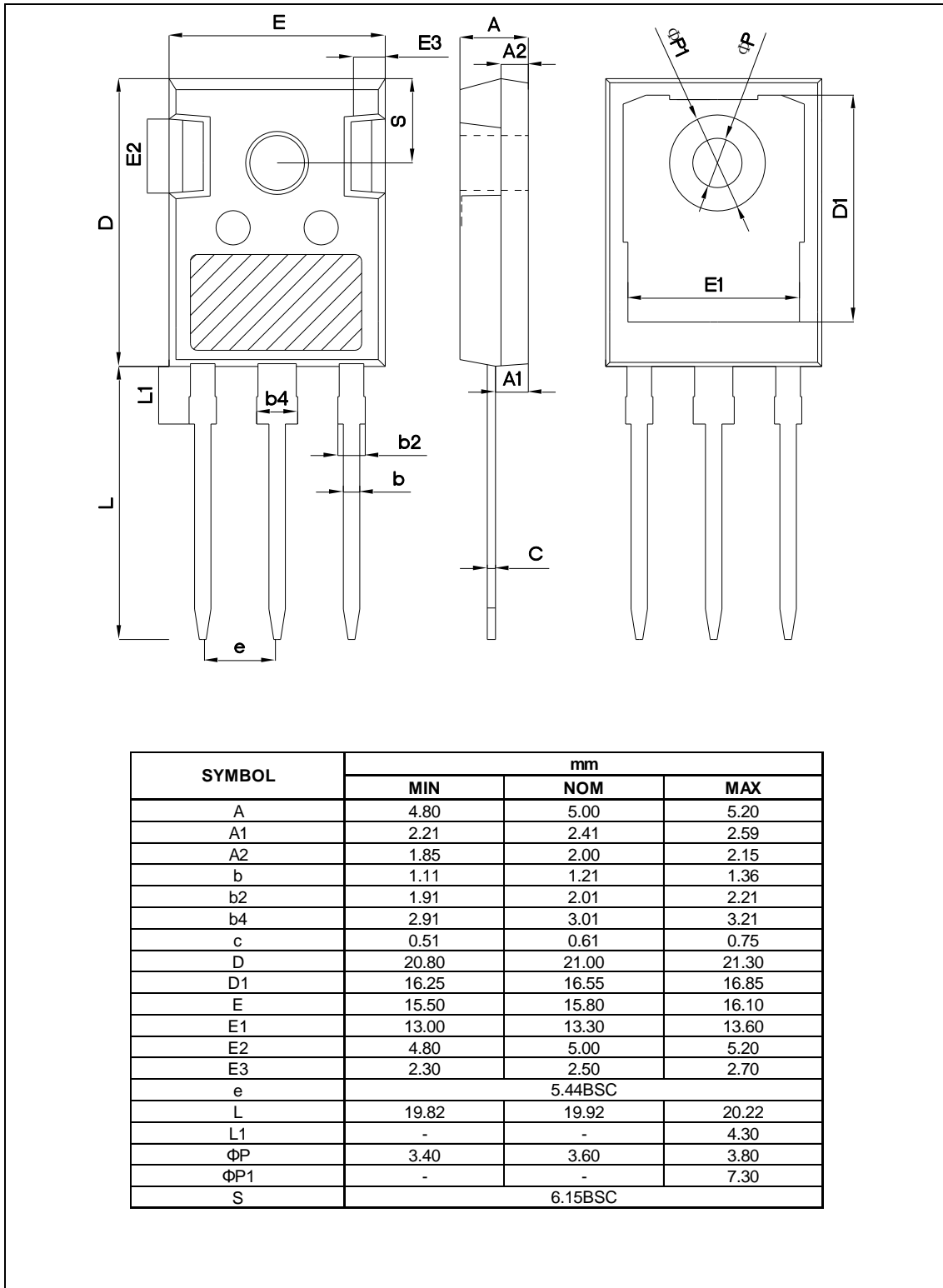
Figure3, TO247 package outline dimension
