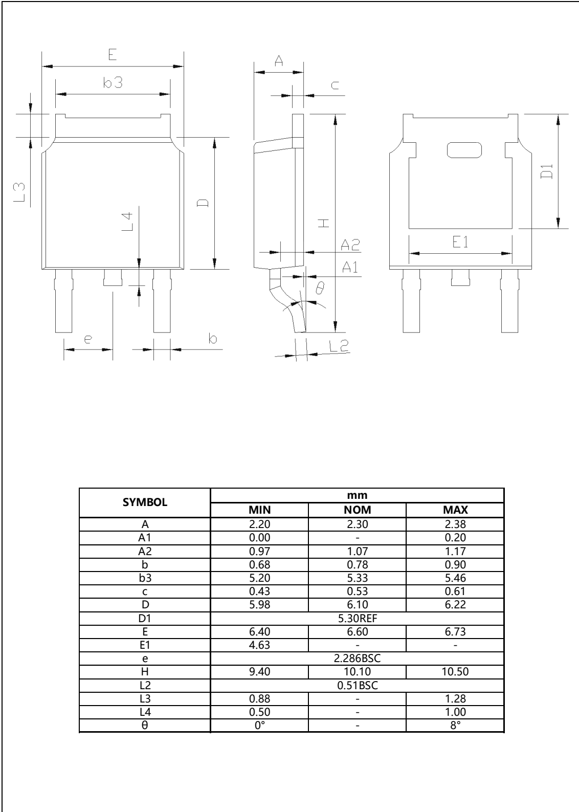
Figure1, Figure1, TO252 package outline dimension
