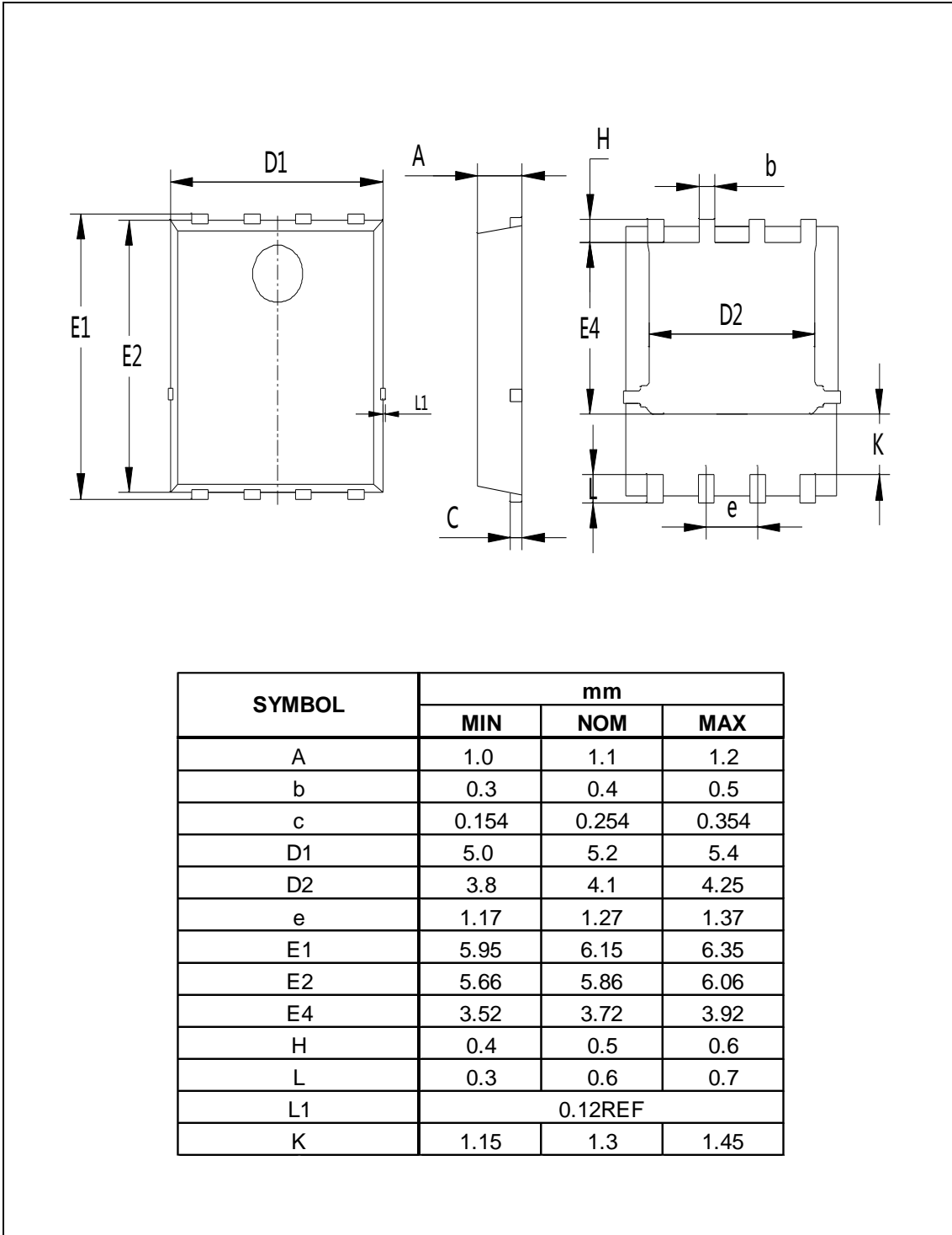
Figure1, PDFN5×6 package outline dimension
