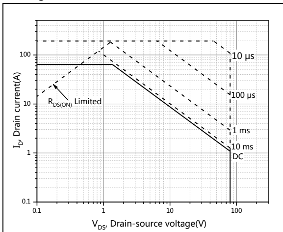
Figure 11, Safe operation area for T_c = 25\text{ °C}
